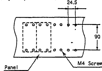
Fig.9 Terminal Arrangement
