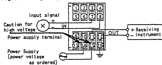
Fig.10 Wiring Diagram
