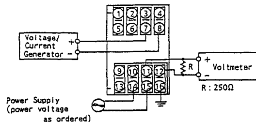
Fig.11 Wiring of Calibration Equipment
